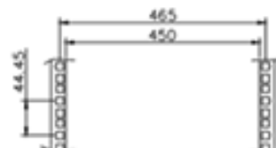
Mounting dimension
